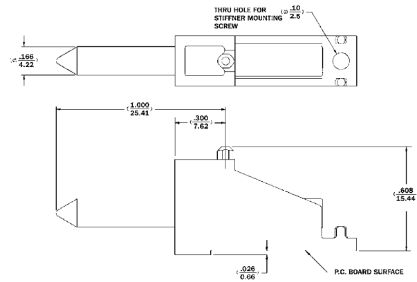
PART No HRG42001 SHOWN
