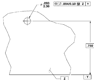
PART No HRG42001 SHOWN
